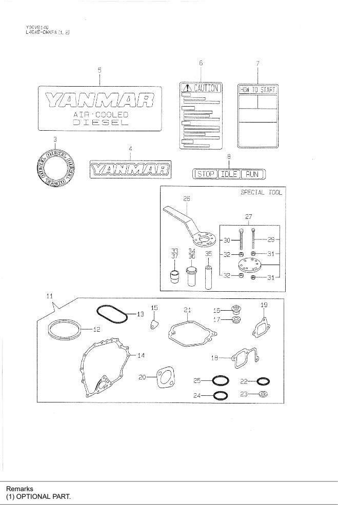
Fig.9. TOOL,LABEL & GASKET SET
